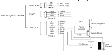
Figure 4-2 Device Wiring
