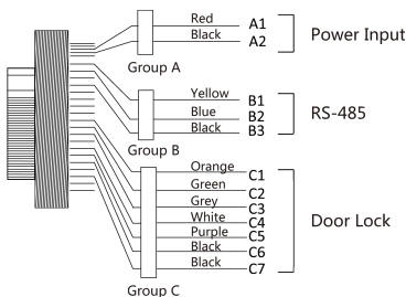
Figure 4-1 Terminal Diagram
