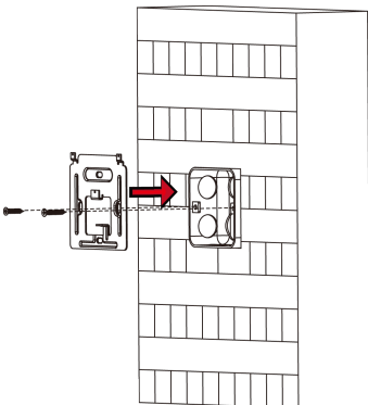
Figure 3-4 Install Mounting Plate
