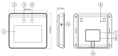
Figure 2-1 Face Recognition Terminal Diagram
