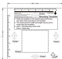
Figure 3-2 Mounting Template
